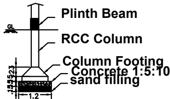
Foundation Detail
