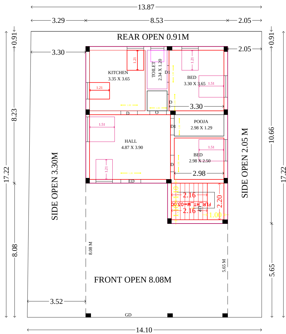
GROUND FLOOR ( NORTH FACING)
