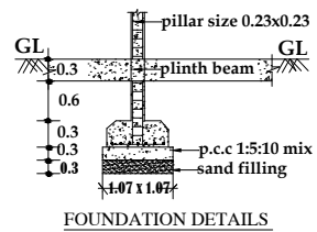
FOUNDATION DETAILS COLUMN FOUNDATION
