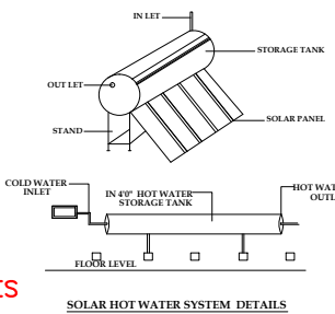
SOLAR HOT WATER SYSTEM DETAILS
