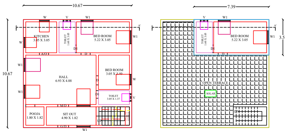
GROUND FLOOR PLAN (NORTH FACING)
