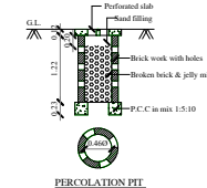
PERCOLATION PIT
