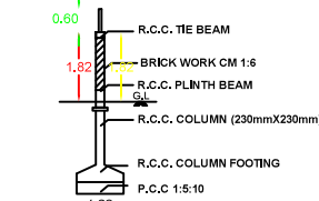
COMPOUND WALL DETAILS
