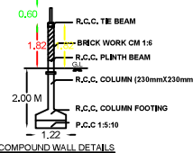
COMPOUND WALL DETAILS
