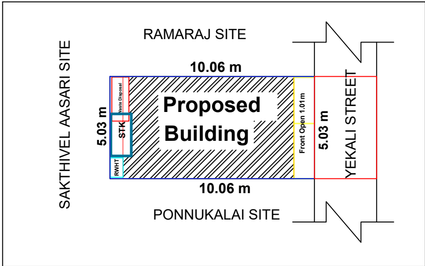
SITE PLAN
