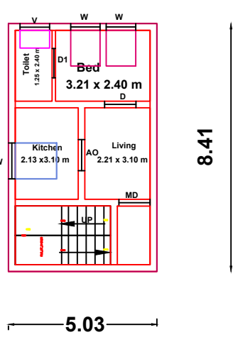
FIRST FLOOR (East Facing)
