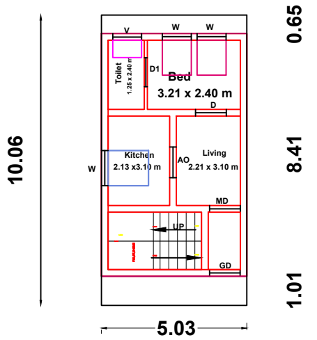
GROUND FLOOR (East Facing)
