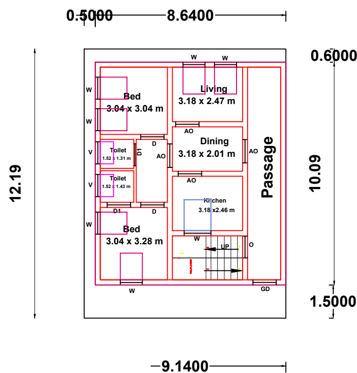
GROUND FLOOR (South Facing)
