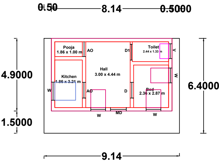
GROUND FLOOR (East Facing)
