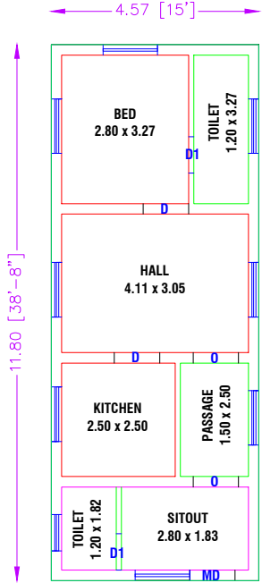
GROUND FLOOR PLAN [EAST FACING]
