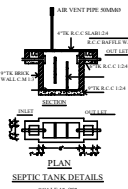
SEPTIC TANK DETAILS
