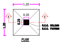
DETAILS OF COLUMN FOOTING
