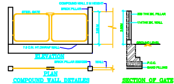
COMPOUND WALL DETAILS
