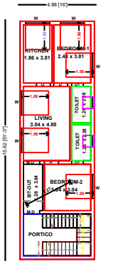
GROUND FLOOR PLAN
