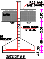
SECTION 'E-E'
