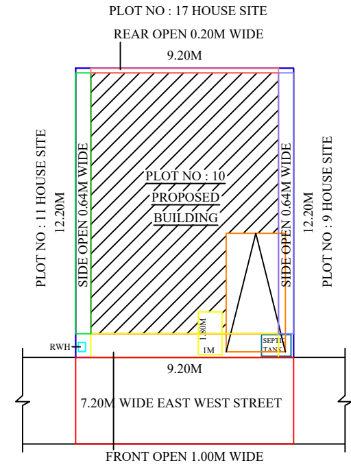
LAY OUT APPROVAL - L.P/AD DTCP(TD) NO : SWP/59/2023
