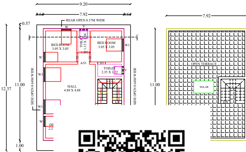
FOOR PLAN
