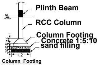
Foundation Detail
