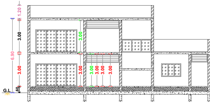
SECTION ON'A-A'
