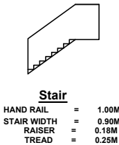
PROPOSED FIRST FLOOR
