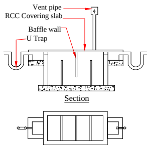
Bath & wash basin pipe line connection is directly connected to the rectangle pit for recycling the waste water.
