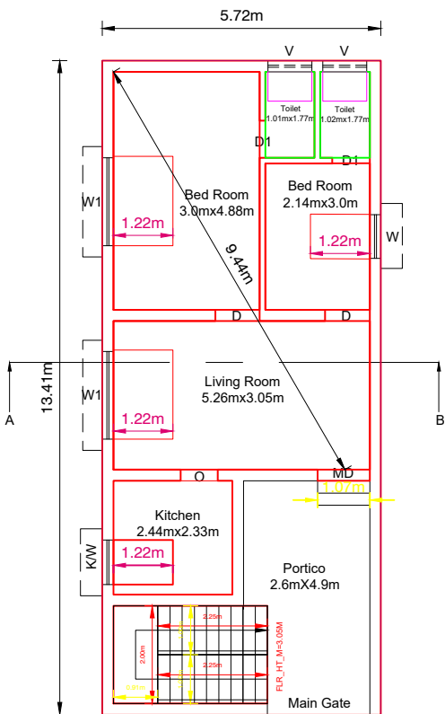
GROUND FLOOR PLAN [EAST FACING]
