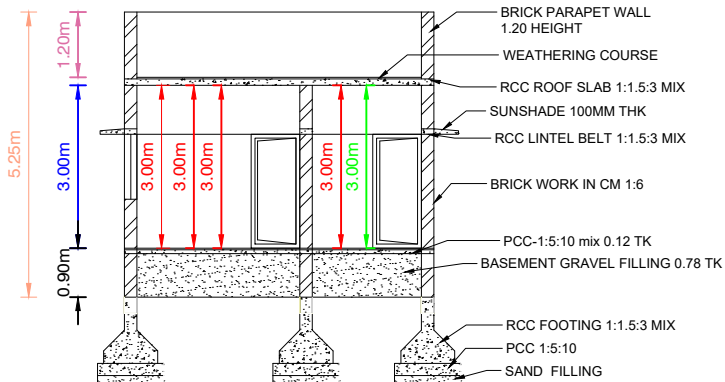
CROSS SECTION - 'AB'
