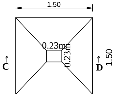
SECTION - 'CD'
