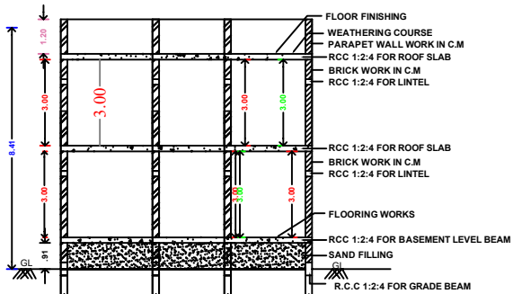
SECTION ON "BB"
