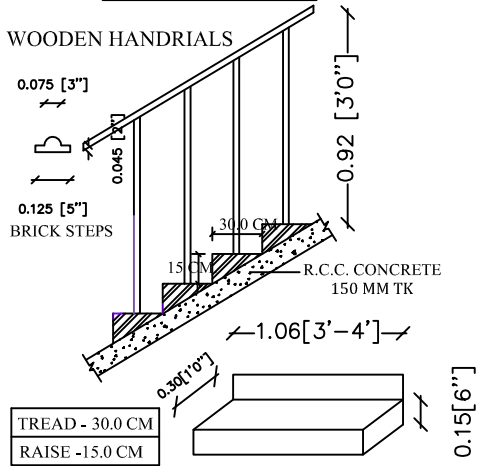
STAIRCASE DETAILS
