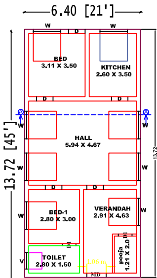
GROUND FLOOR PLAN (WEST FACING)
