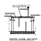
SEPTIC TANK SECTION
