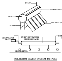
SOLAR HOT WATER SYSTEM DETAILS
