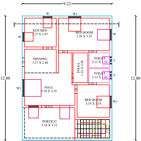
GROUND FLOOR PLAN (NORTH FACING)
