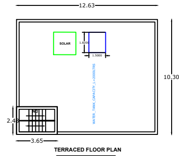
TERRACED FLOOR PLAN
