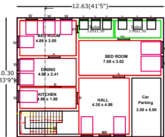
GROUND FLOOR PLAN ( EAST FACING)
