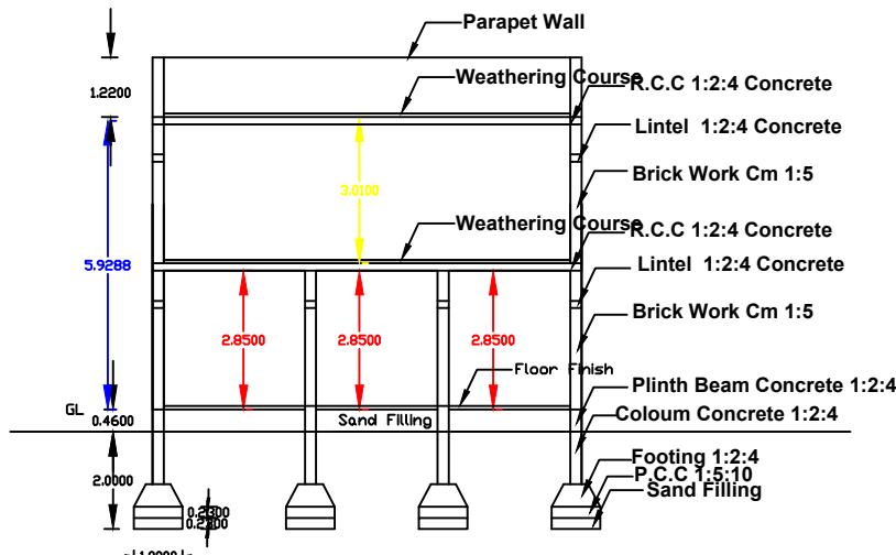
Section Section - AA
