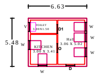
GROUND FLOOR PLAN
