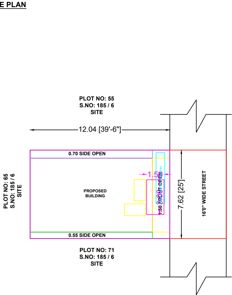
SITE PLAN
