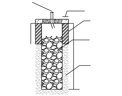
RAIN WATER HARVESTING PIT DETAILS
