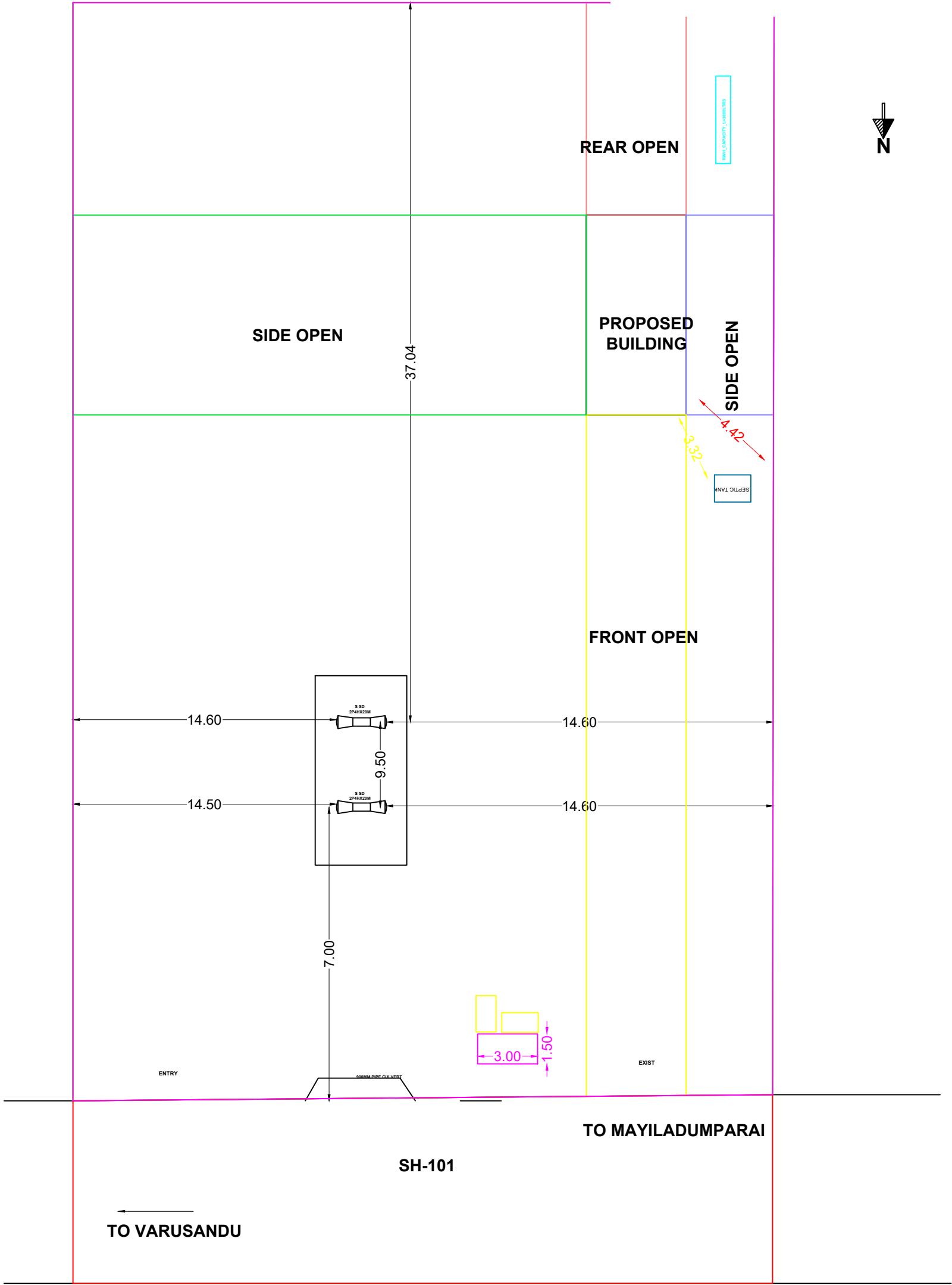
SITE PLAN
