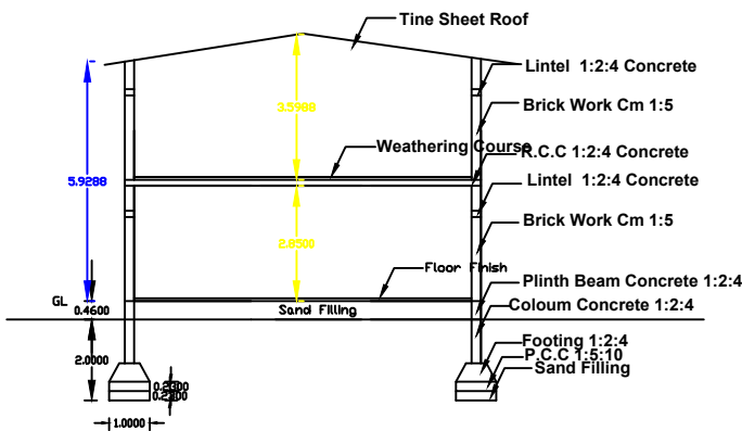
Section Section - AA
