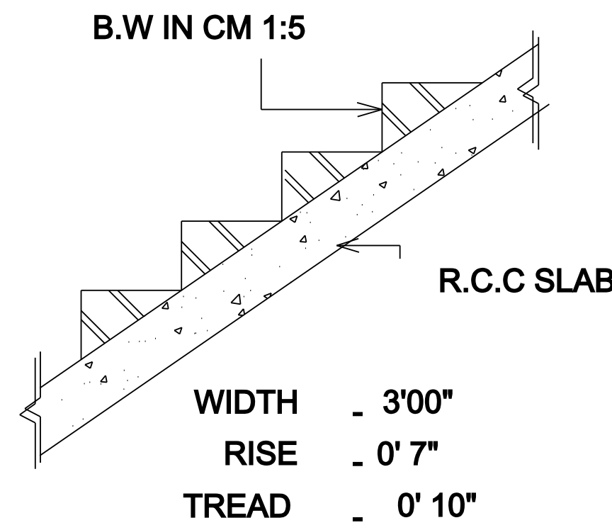
STAIR DETAILS
