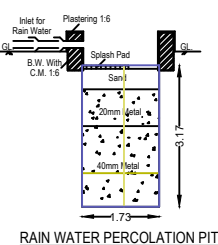
RAIN WATER PERCOLATION PIT
