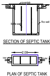
PLAN OF SEPTIC TANK
