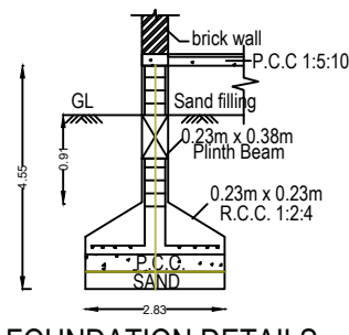
FOUNDATION DETAILS
