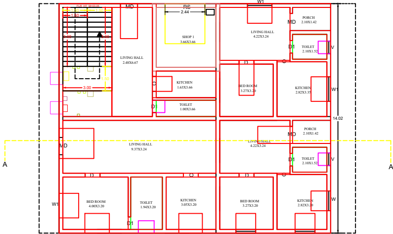
PROPOSED GROUND FLOOR
