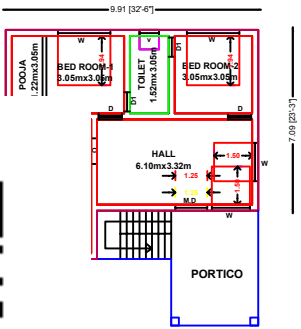
ND FLOOR PLAN
