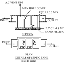
DETAIL OF SEPTIC TANK (Not to scale)
