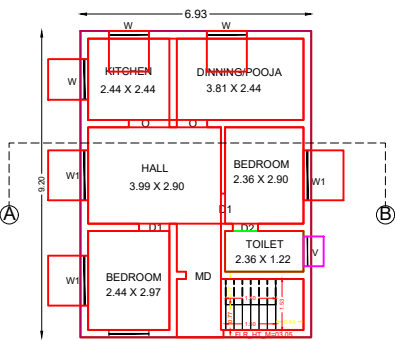
PROPOSED GROUND FLOOR PLAN (NORTH FACING)
