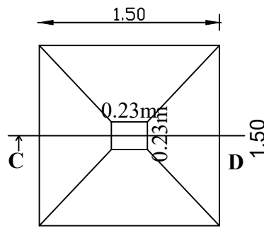
SECTION - 'CD' FOUNDATION DETAIL - A
