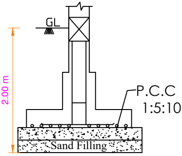
Isolated Footing -A (1.50X1.50) (Not to Scale)
