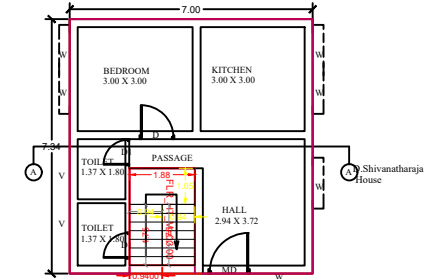
FIRST FLOOR PLAN (Existing Building)
