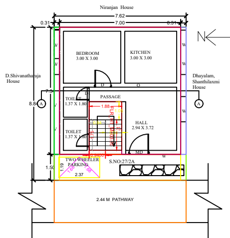
SITE CUM GROUND FLOOR PLAN (Existing Building)
