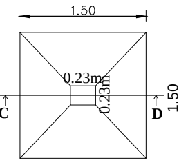
SECTION - 'CD' Plan
