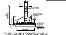
TYP. DET. COLUMN & FOUNDATION FOOTING
