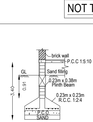
FOUNDATION DETAILS
