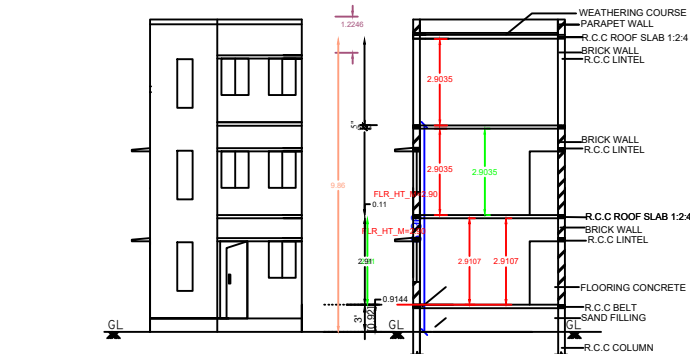
FRONT ELEVATION SECTION ON AA
