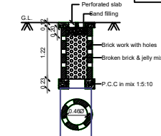
PERCOLATION PIT FOR 30sq.m. (Scale:- 1:50)
