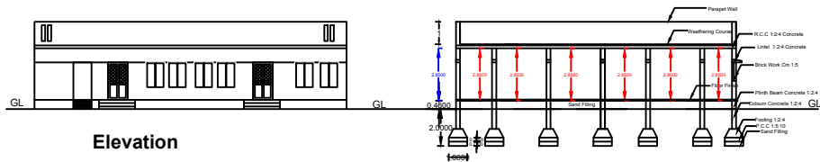
Section Section - AA
