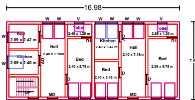
Ground Floor Plan (East Facing)
