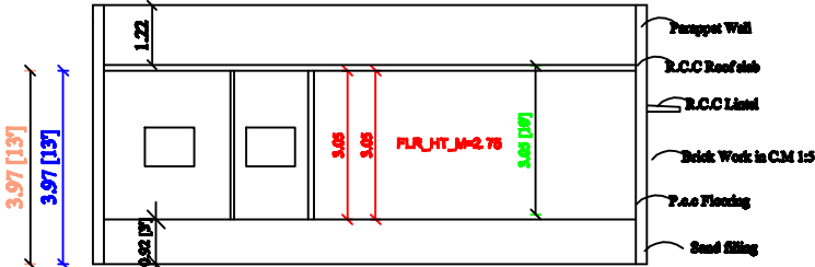
SECTION ON"AA"
