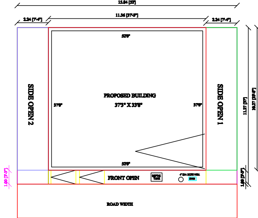
SITE PLAN
