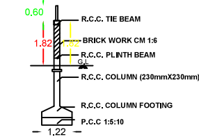
COMPOUND WALL DETAILS
