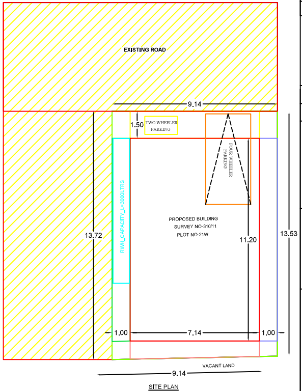
SITE PLAN
