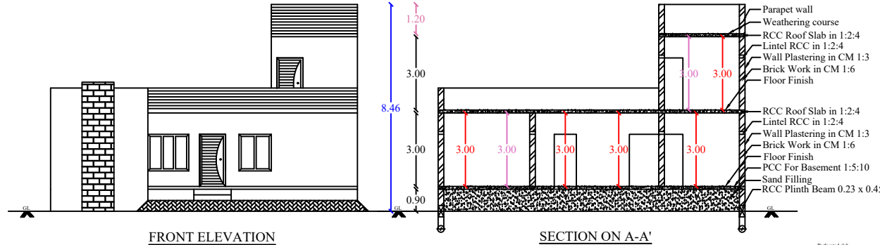
FRONT ELEVATION
