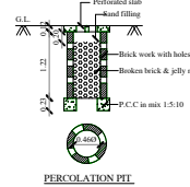
PERCOLATION PIT
