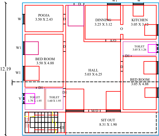
GROUND FLOOR PLAN (WEST FACING)
