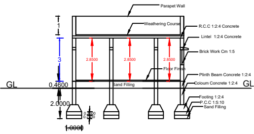
Section Section - AA
