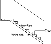
DETAILS OF STAIR CASE
