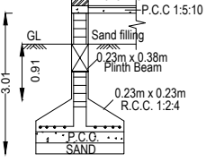
FOUNDATION DETAILS
