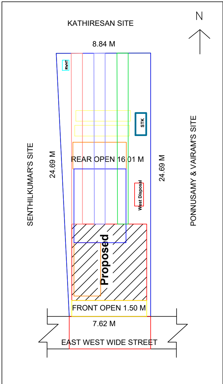
SITE PLAN
