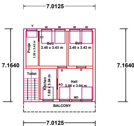
GROUND FLOOR PLAN ( EAST FACING )
