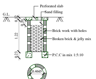
PERCOLATION PIT
