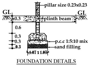
FOUNDATION DETAILS
