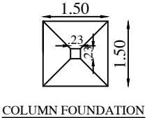
COLUMN FOUNDATION
