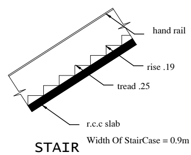
STAIR Width Of StairCase = 0.9m
