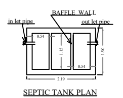
SEPTIC TANK PLAN
