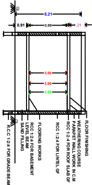
SECTION ON AA
