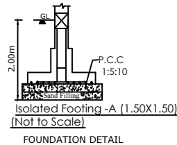
FOUNDATION DETAIL
